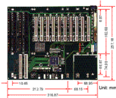
14-Slot (10xPCI) PICMG Backplane
