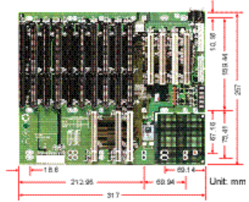
14-Slot (4xPCI) PICMG Backplane
