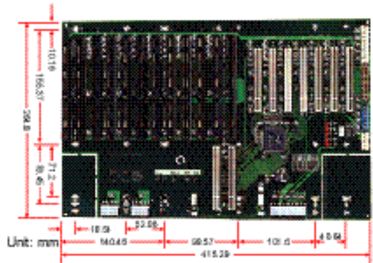
19-Slot (7xPCI) PICMG Backplane
